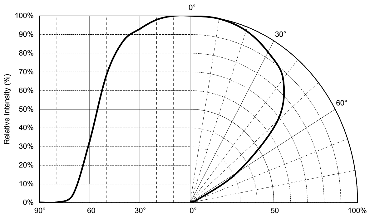
Fig 2. Radiation Characteristics
